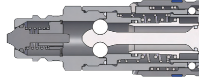
HT-AG-Series Flush Face ISO16028 Coupler x ISO7241-A AG Plug Adapter
