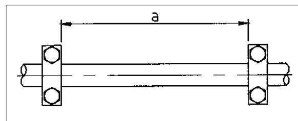
Recommended fastening distances (to DIN 24346)
